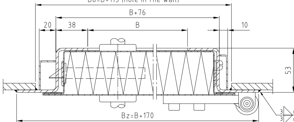
Bo=B+115 (hole in the wall)
